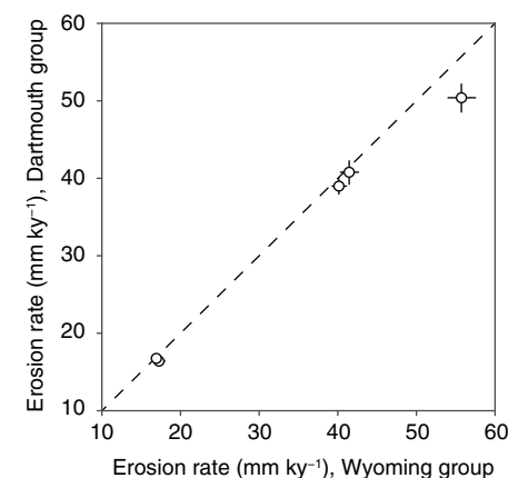
Figure 6. Erosion rates inferred from cosmogenic nuclide concentrations in stream sediment sampled at same locations but two different times and processed at two different laboratories. Erosion rates of samples collected in 2004–2006 and processed at Dartmouth College agree closely with erosion rates of samples collected in 2009–2010 and processed at the University of Wyoming. Error bars include relative error from analytical uncertainty. Measurements from four of the five duplicate analyses agree within one standard error and all of the data lie close to a 1:1 line.
