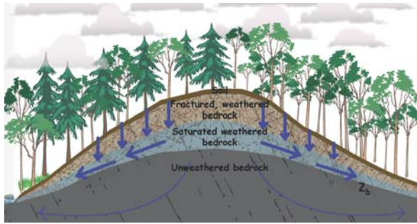
Figure 4. Idealized cross-section through the Rivendell hillslope (left) and profiles (right) showing vertical structure and seasonal rapid injection of winter rain via fracture flow to a perched water table as soil and saprolite and weathered bedrock more slowly gain moisture (Salve, et al., 2012). Z_b in the left figure is the boundary to fresh bedrock (Rempe and Dietrich, 2012)
