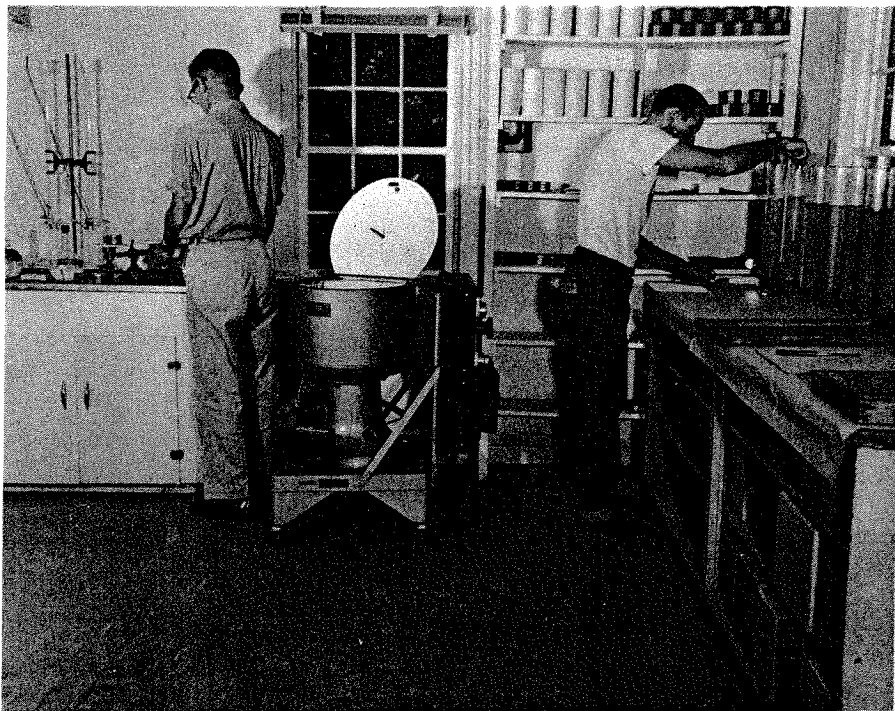
Figure 15.-In the laboratory a man on the left is weighing the soil sample while the man on the right determines texture (percent of sand, silt, and clay). The centrifuge that stands between them is used for studying soil moisture.
