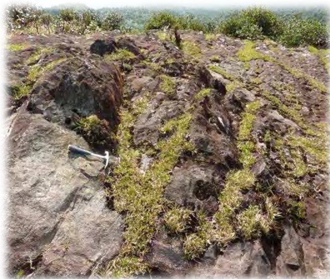
Geoscientists are studying erosion on El Yunque, a hard-headed "cap" on the island.
