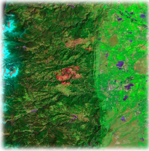
Location of Boulder Creek, and tributary Fourmile Creek, with red burn scar from a wildfire.
